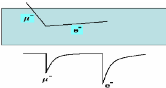
FIGURE 5. Typical signature of the nuclear (scintillator) capture of a negative muon followed by its decay emitting an electron (plus two neutrinos). The two serial (inverse) peaks correspond to the signal of the muon and electron respectively.
